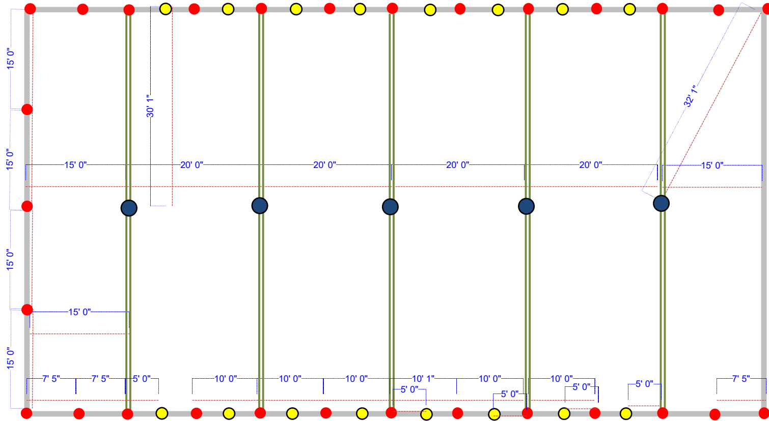
30' x 110' Pole Tent Standard & Wind - Pole Placements
